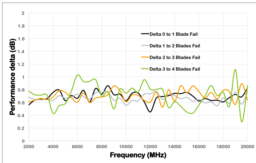
Figure 2 | Comparative degraded performance of a 16-blade amplifier.
