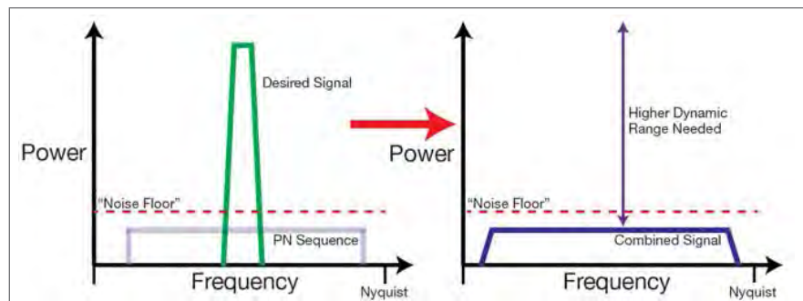
Figure 3 | Direct Sequence Spread Spectrum systems require a wide receiver bandwidth and high dynamic range as the signal band of interest is combined with pseudorandom noise (PN) to push the communication into the noise floor.
