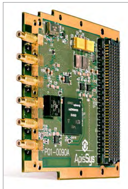
Figure 3 | The AF209 from ApisSys is based on the VITA 57 FMC standard.
