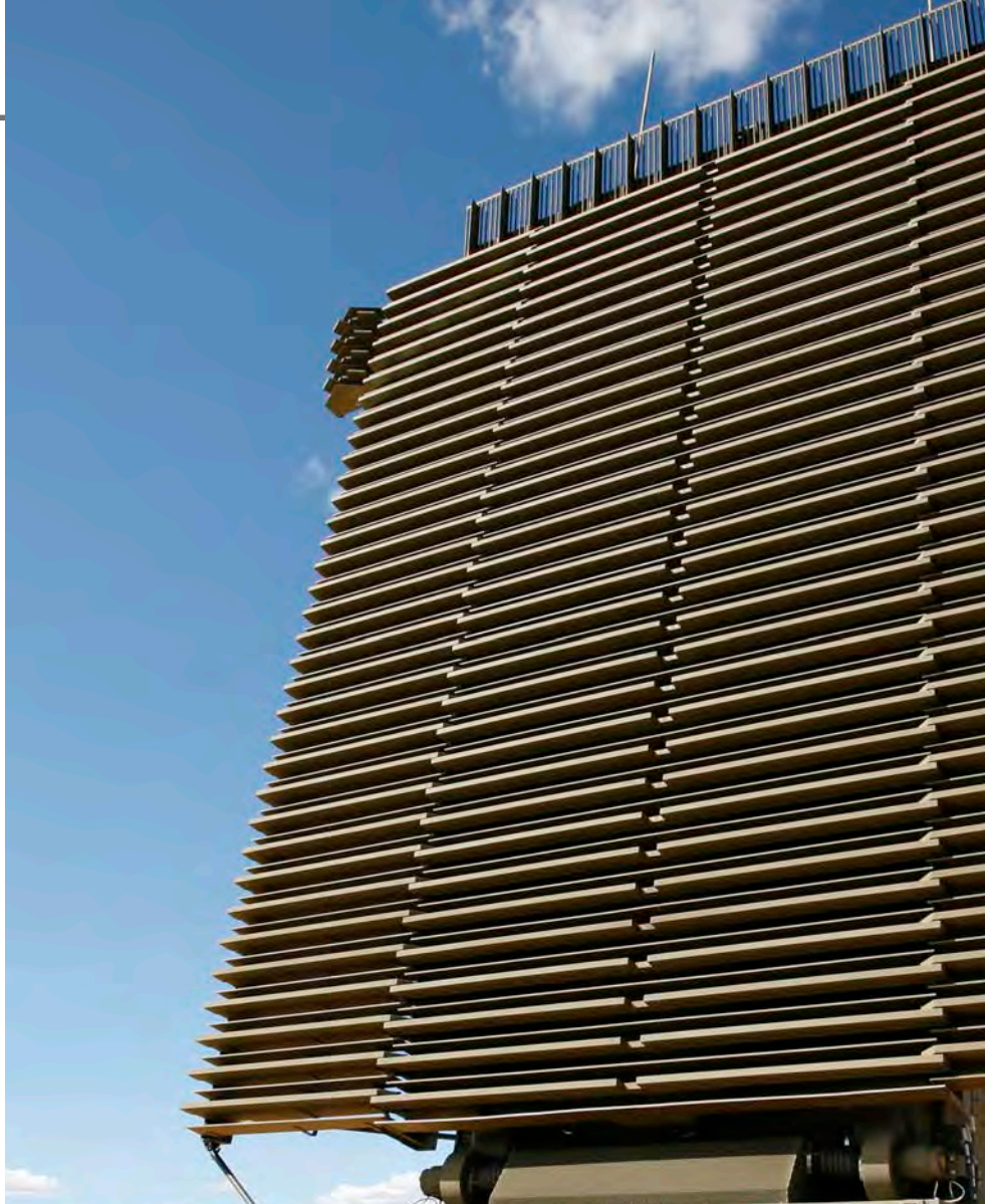
Lockheed Martin's Digital Array Row Transceiver (DART) is a combined transmit-and-receive line replaceable unit (LRU) with gallium nitride transmit/receive modules. Photo courtesy of Lockheed Martin.
