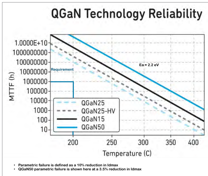
Figure 1 | GaN lifetime vs. junction temperature.
