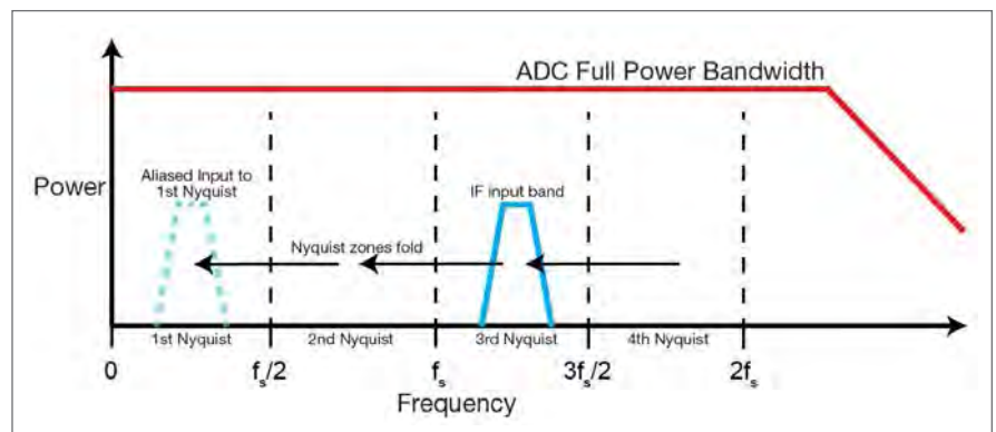
Figure 1 | Wide ADC full-power bandwidth enables the use of higher order Nyquist bands. Band pass filtering of the unused Nyquist zones is mandatory to remove unwanted signal energy that could potentially fold back into the first Nyquist, thereby impacting dynamic range.
