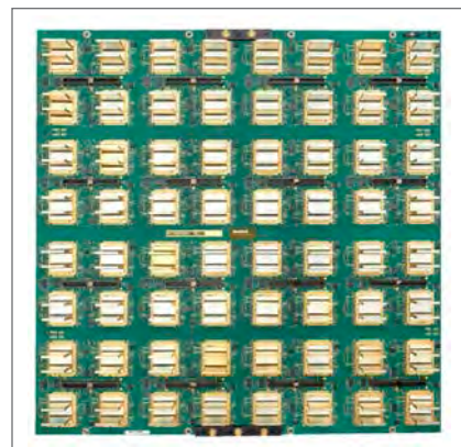
Figure 1 | Pictured is a SPAR Tile developed by MACOM. Photo courtesy of MACOM.
