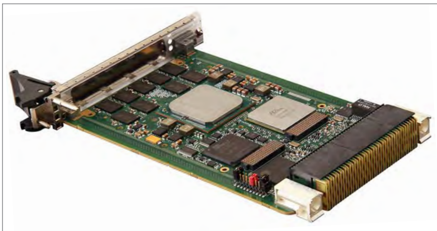
Figure 2 | Curtiss-Wright's 3U OpenVPX CHAMP-XD1 is a SWaP-optimized DSP engine module that leverages the performance specs of Intel's Xeon processor D architecture for EW applications.
