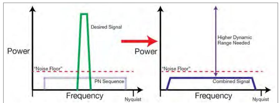
Figure 2 | Direct Sequence Spread Spectrum systems require a wide receiver bandwidth and high dynamic range as the signal band of interest is combined with pseudorandom noise (PN) to push the communication into the noise floor.
